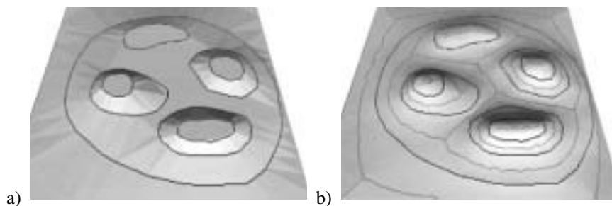
a) b) Figure 17. Triangulation of several small hills: a) triangle-based interpolation, b) Sibson interpolation with slopes
