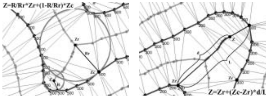
Figure 6. Estimating skeleton heights: a) from circumradii; b) from valley length
