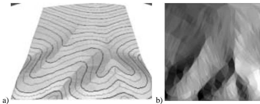
Figure 8. Adding skeleton points to Fig. 7: a) perspective view; b) vertical view
