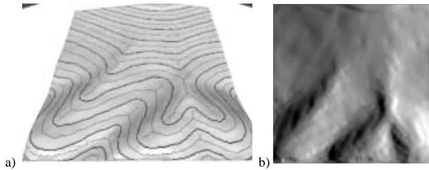
Figure 15. Sibson interpolation using slopes and smoothing function at data points: a) perspective view; b) vertical view
