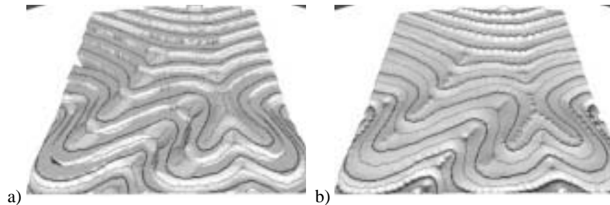
Figure 10. Gravity model interpolation: a) with small radius b) with large radius
