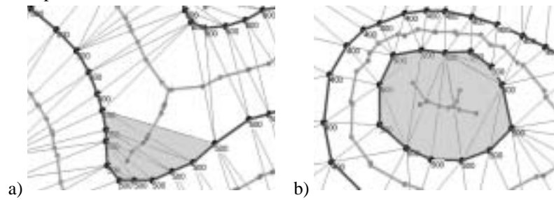
Figure 4. Skeleton and "flat triangles": a) ridge; b) summit
