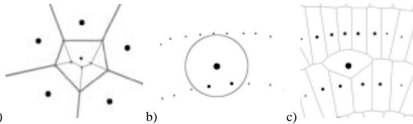
Figure 11. a) Sibson interpolation; b) neighbour selection using a counting circle; c) neighbour selection using Voronoi neighbours
