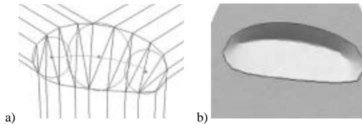
Figure 5. Triangulation of a summit: a) skeleton and circumcentres; b) elevation model after adding skeleton vertices with assigned height values
