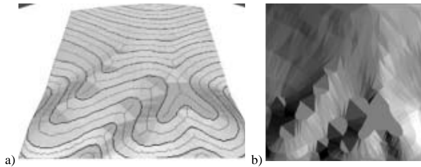
Figure 7. Triangle-based interpolation: a) perspective view; b) vertical view
