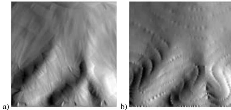
Figure 16. Adding slopes at data points: a) triangle-based interpolation; b) gravity interpolation
