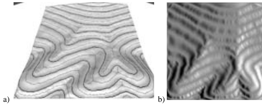
Figure 13. Adding smoothing to Fig. 12: a) perspective view; b) vertical view
