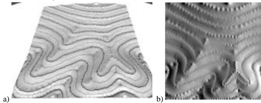
Figure 9. Interpolation using the gravity model with medium radius: a) perspective view; b) vertical view
