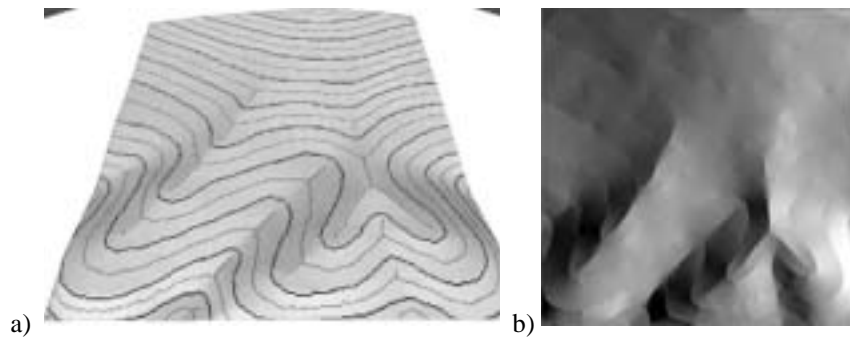
Figure 12. Sibson interpolation: a) perspective view; b) vertical view
