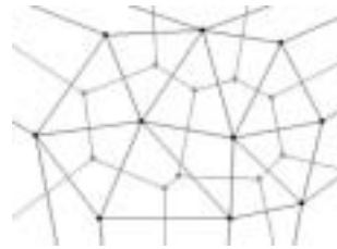
Figure 1. Delaunay triangulation and Voronoi diagram
