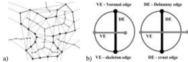
Figure 2. Crust and skeleton: a) crust (thick black lines) and skeleton (thick grey lines); b) crust/skeleton test
