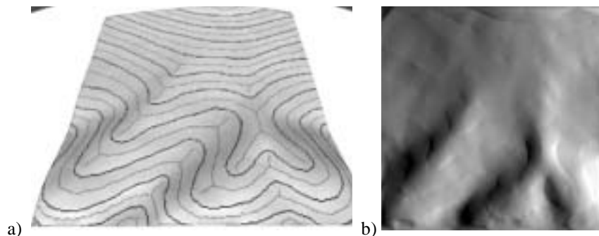
Figure 14. Sibson interpolation using slopes at data points: a) perspective view; b) vertical view
