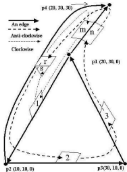
Figure 18. Use “SEMV” to split the edge
