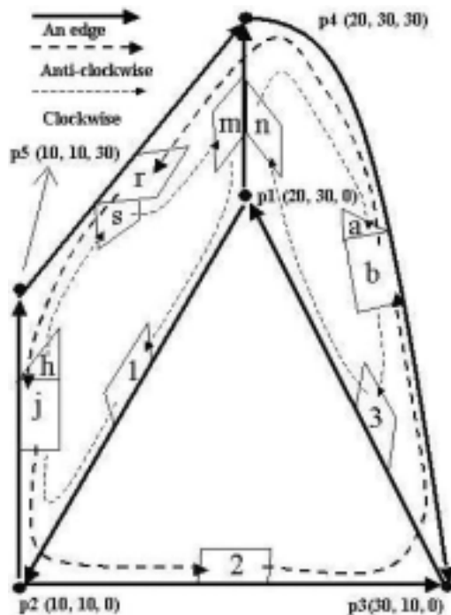
Figure 20. Make a new face using “MEF”
