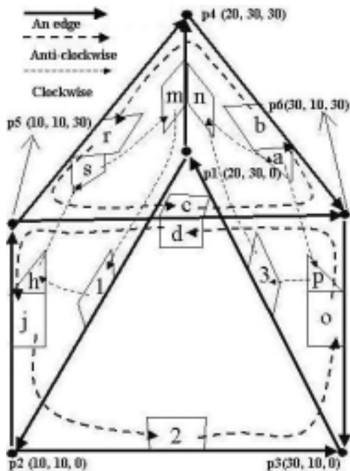
Figure 22. Use “MEF” to split a face
