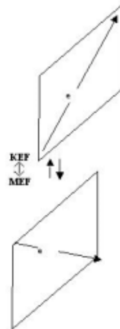
Figure 3.2 Swap
