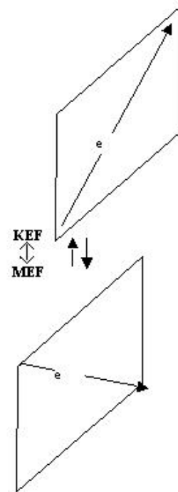
Figure 2.2 Splice
