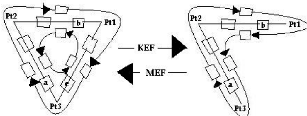
Figure 2.3 Before KEF
