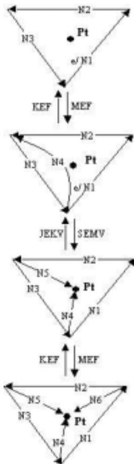
Figure 3.1 Insert Point
