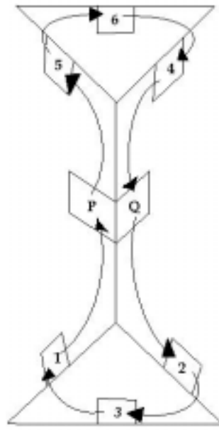
Figure 4.3 MEHKF
