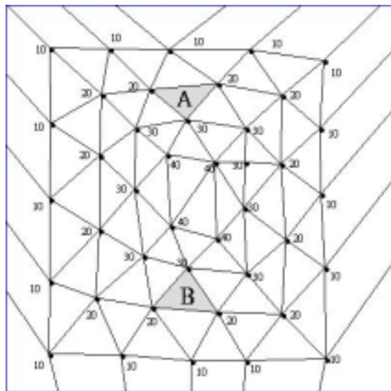
Figure 4.1 TIN model with two selected triangles
